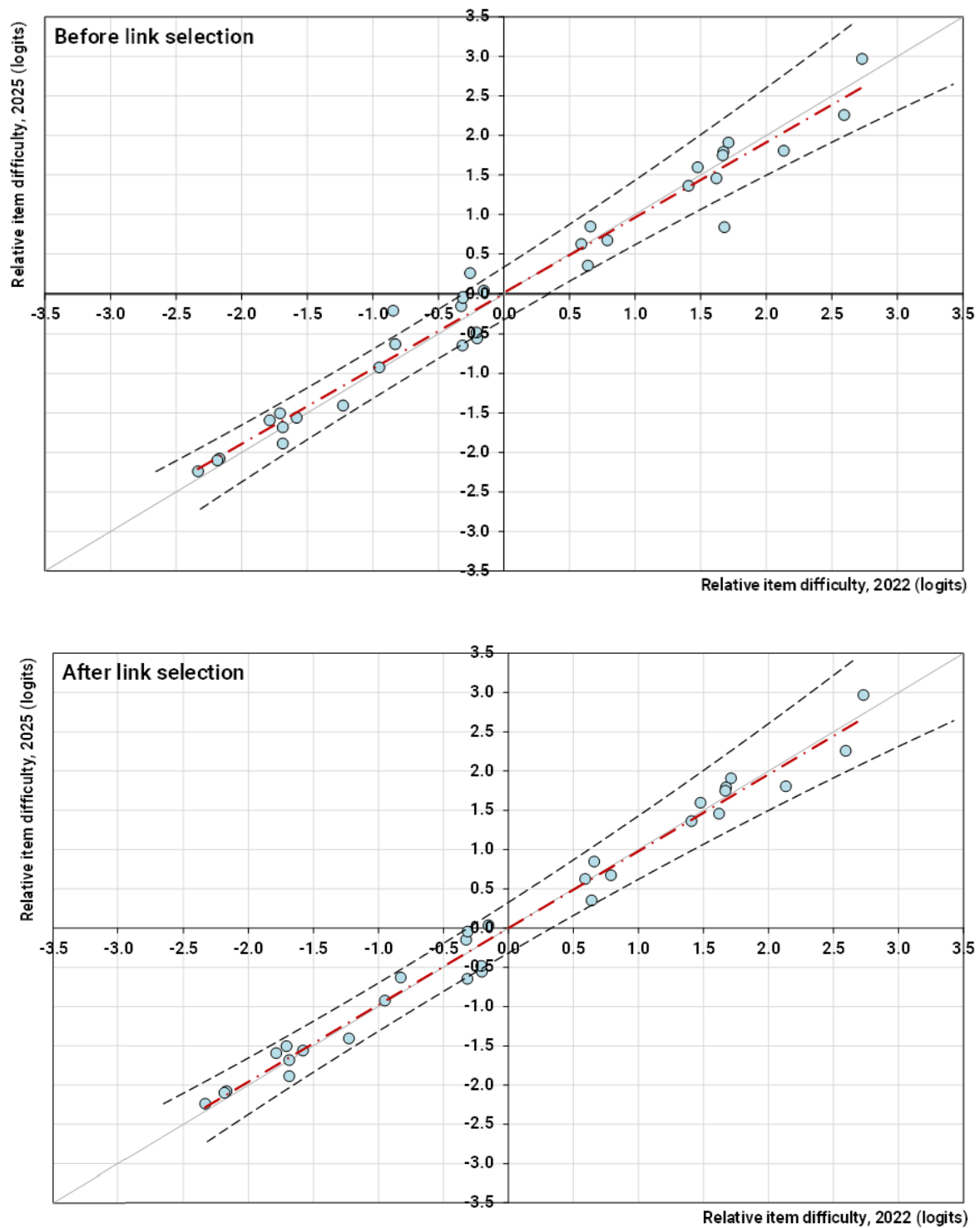
Figure 5.3: Scatter plots comparing relative item difficulties of trend module items from 2022 and 2025 at Year 6, for (top) before link selections were made and (bottom) after link selections were made, removing 3 out of 33 items as horizontal links, leaving 30 remaining links.
