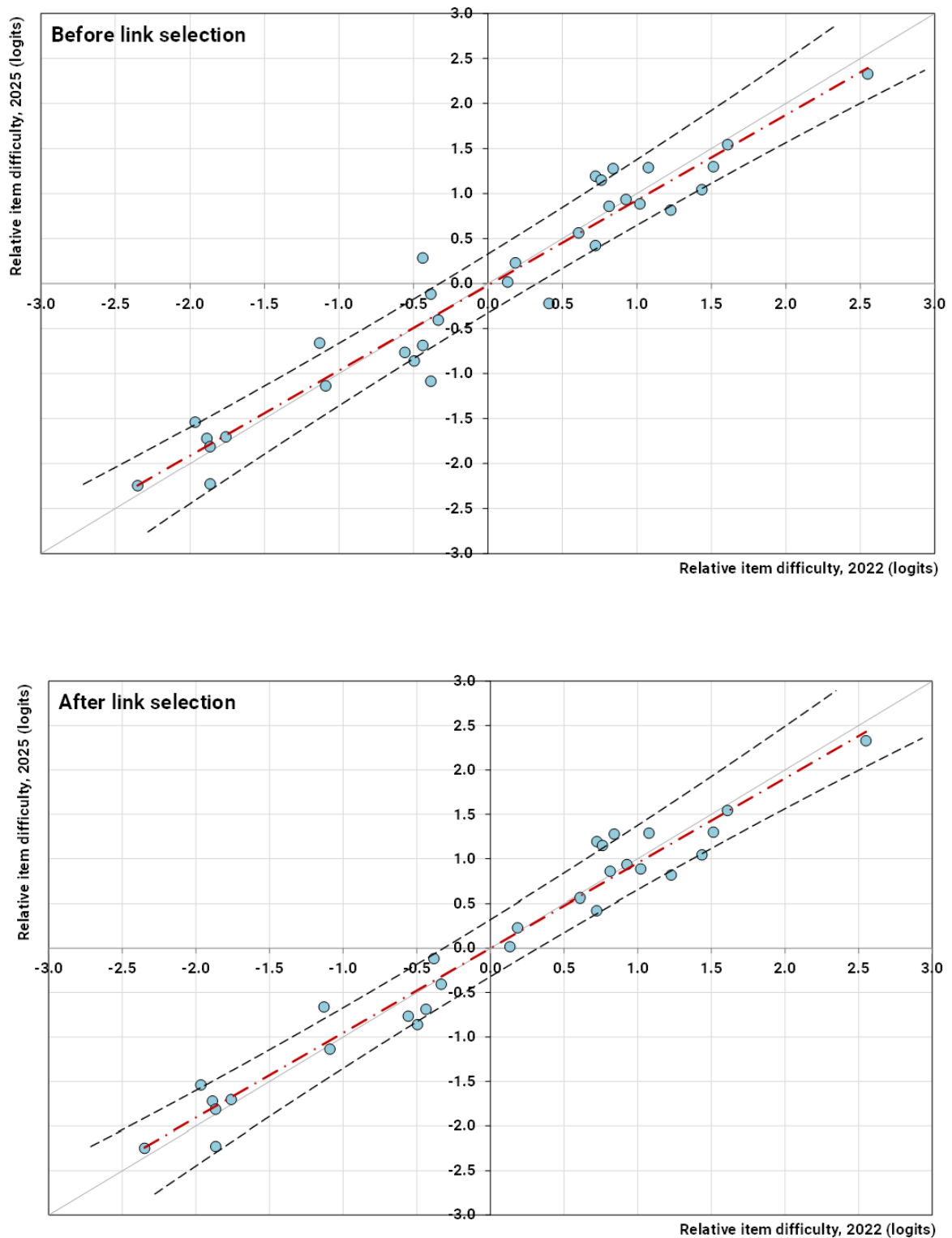
Figure 5.5: Scatter plots comparing relative item difficulties of trend module items from 2022 and 2025 at Year 10, for (top) before link selections were made and (bottom) after link selections were made, removing 3 out of 32 items as horizontal links, leaving 29 remaining links.
