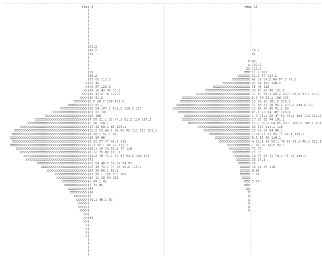
Figure 5.2: Item maps for Year 6 and Year 10
