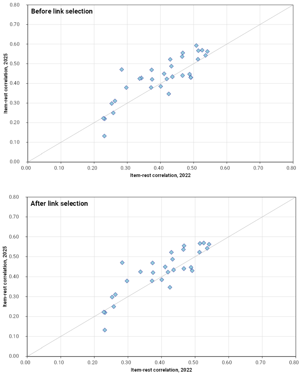
Figure 5.6: Scatter plots comparing item-rest correlations of trend module items from 2022 and 2025 at Year 10, for (top) before link selections were made and (bottom) after link selections were made, removing 3 out of 32 items as horizontal links, leaving 29 remaining links.
