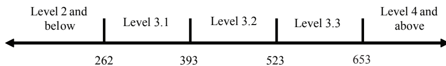
Figure 4.1 Cut-off scores
